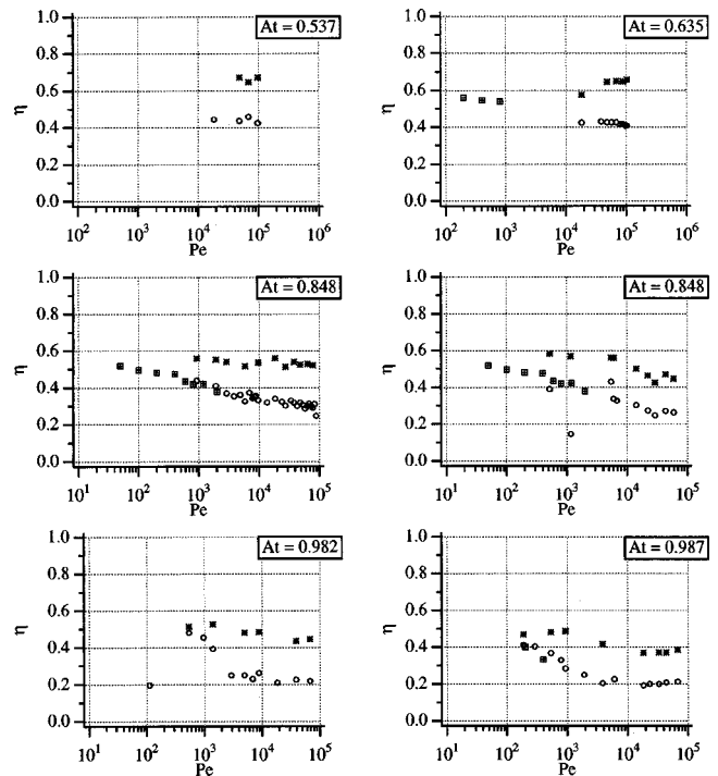
FIG. 4. Surface efficiency \eta_{sur} (*) and volume efficiency \eta_{vol} (O) as a function of the Pe for five different At values. The square symbols were obtained from the simulations of Chen and Meiburg (Ref. 10). Graphs (c) and (d) correspond to the same At , but the different fluid combinations of Figs. 3(a) and 3(b), respectively.
