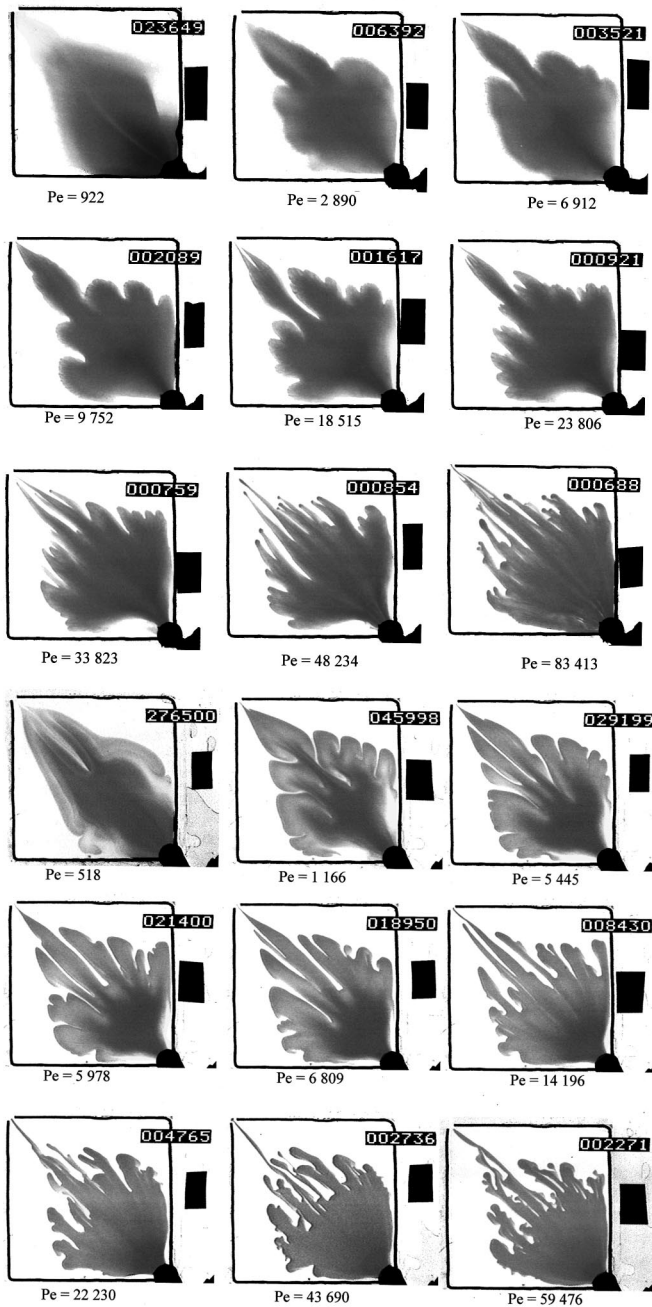
FIG. 3. (a) Fingering patterns at the breakthrough time t_{end} for different Peclet numbers. A water-dye mixture displaces a glycerin-water mixture of concentration c_g = 66.4\% . At = 0.848 . (b) Fingering patterns at the breakthrough time t_{end} for different Peclet numbers. A glycerin-water-dye mixture of concentration c_g = 76.9\% displaces a glycerin-water mixture of concentration c_g = 96\% . At has the same value as in (a).
