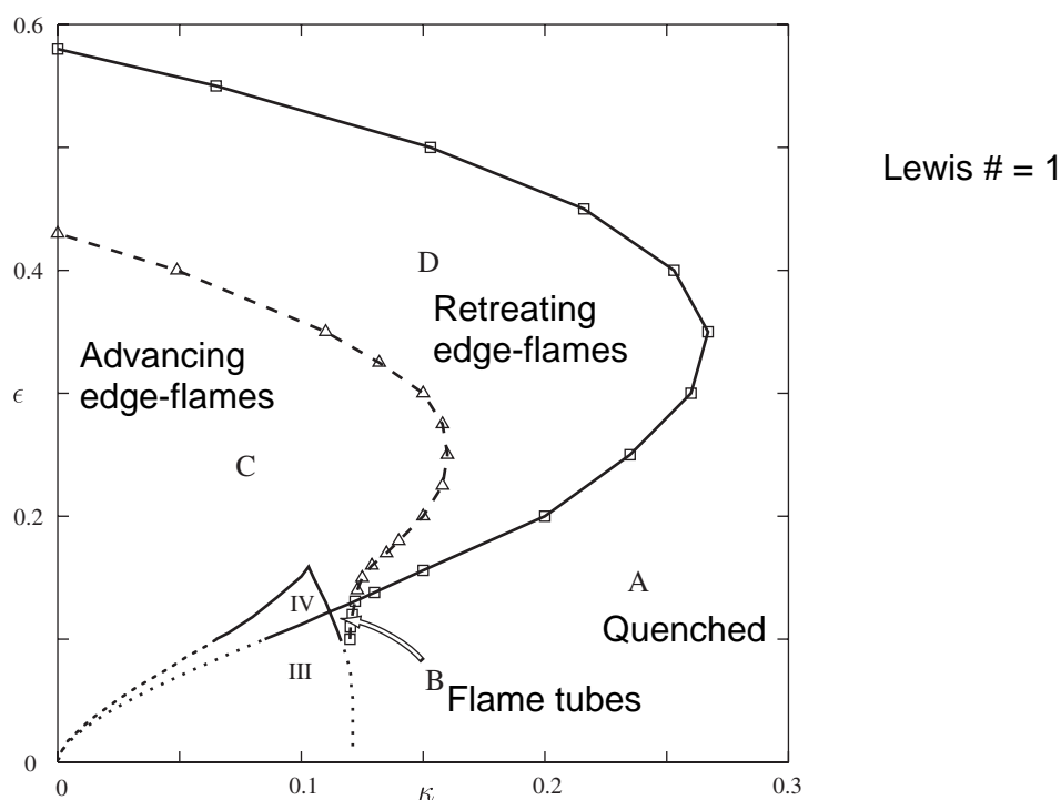
Figure 14. Regimes of flame-edge propagation under strain and heat loss.
