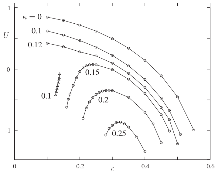
Figure 9. Propagation speed versus \epsilon for selected values of \kappa .
