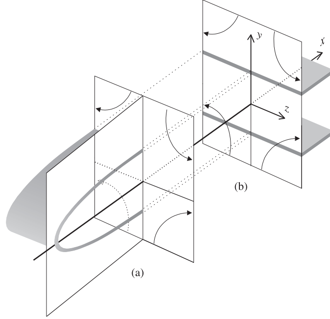
Figure 1. The counterflow configuration: (a) a two-dimensional flame-edge and (b) planar twin-flames.
